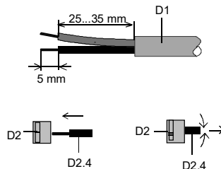
figure 6: Connecting / Disconnecting bus cables
