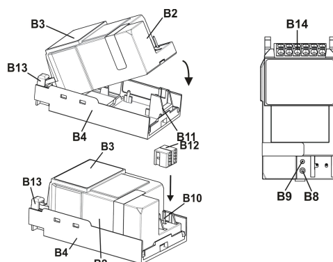
figure 3: Mounting of an RL module
