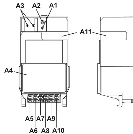
figure 2: Location / Function of the Display and Operating Elements
